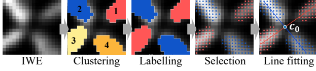
Figure 6. Corner initialization procedure.
