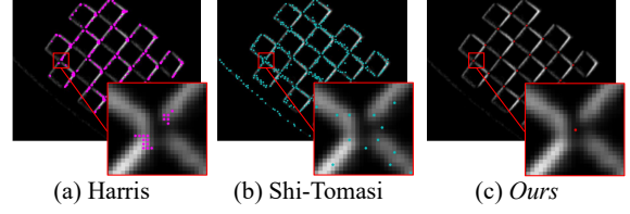
Figure 4. Comparison with conventional methods. Harris [21] and Shi-Tomasi [42] fail under event data, whereas the proposed method achieves accurate and stable localization.
